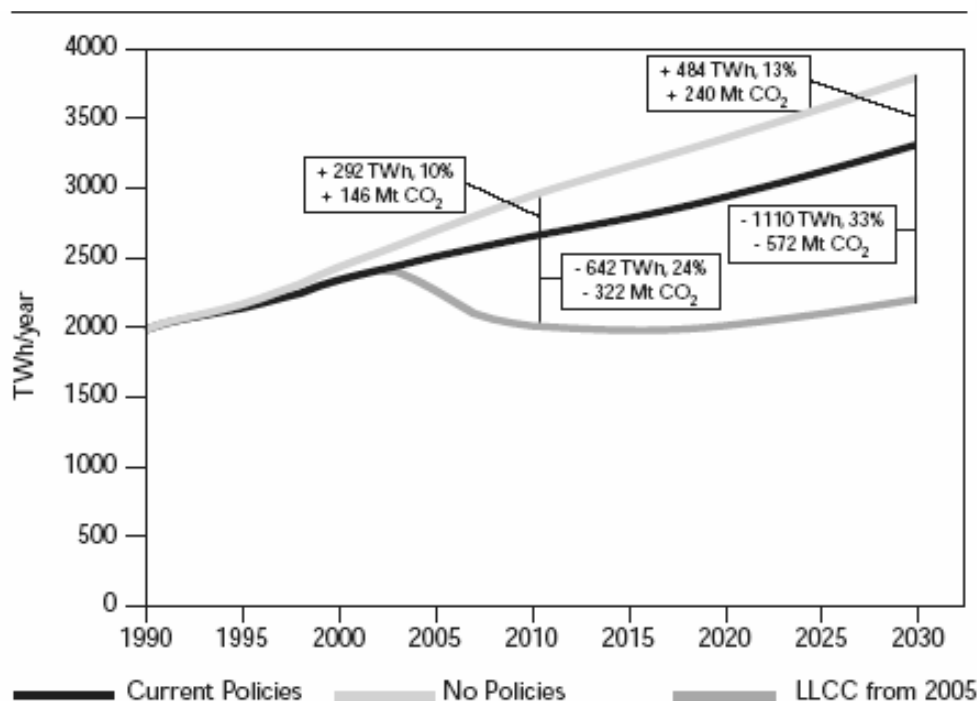
Figure 1: Residential electrical appliance electricity consumption under No Policy, Current Policy and Least Life-Cycle Cost 2005 scenarios in IEA countries, 1990 to 2030
