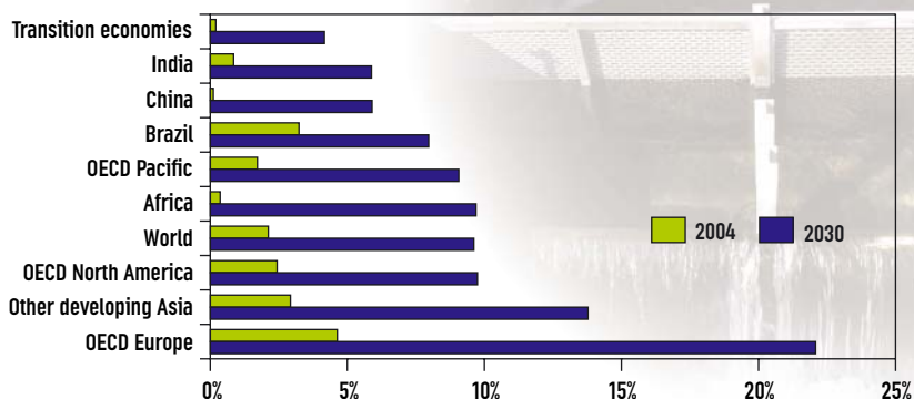
Figure 7 • Shares of non-Hydro Renewable Energy in Electricity Generation by Region
